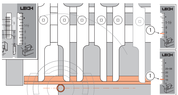
16-12 With the finger assembly (including the sliding dovetail fence) on the support brackets in the HB TAILS mode, set the scale to 7/16" [11mm] ①. Make sure the finger assembly is level and sitting flush on top of the board. The HB TAILS scale was not designed for this operation, but with this setting the routed slot will be close to centered on the slot line.
