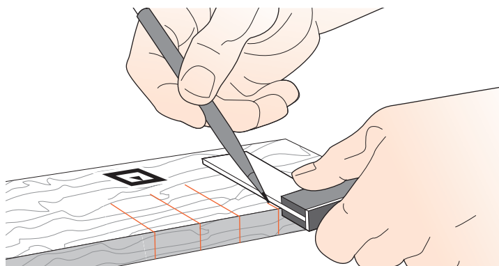
16-8 On the test slot board only, square the marks across the face.
