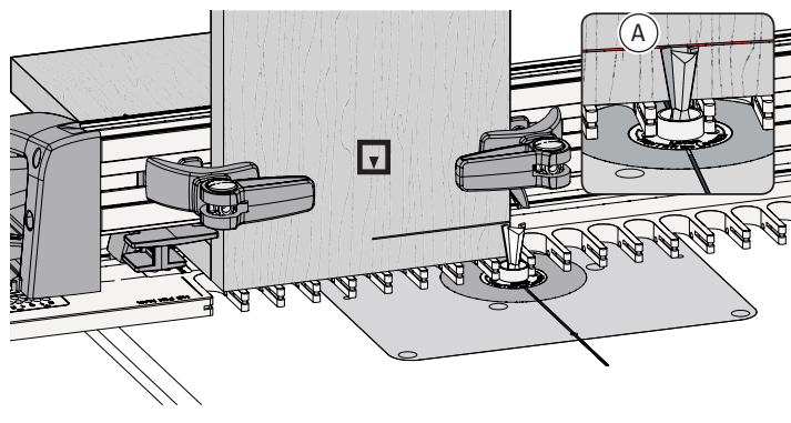
8-13 Position the jig close to the dovetail bit and adjust the bit height until the bit tip is touching the center of the line (A). ⚠ Double check that the bit still rotates freely. Note: Make sure you are using the e10 eBush set on 5.
