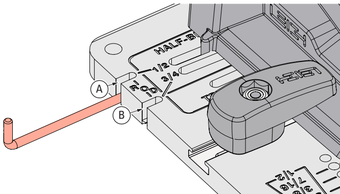
9-12 The Stop Rod. For tail boards (sides) from \frac{3}{8} " [9mm] to \frac{5}{8} " [16mm] thick, insert the stop rod in the \frac{1}{2} " slot (A). Note: For tail boards \frac{1}{16} " [17.5mm] thick or greater, the stop rod is stored in the \frac{3}{4} " slot (B).
