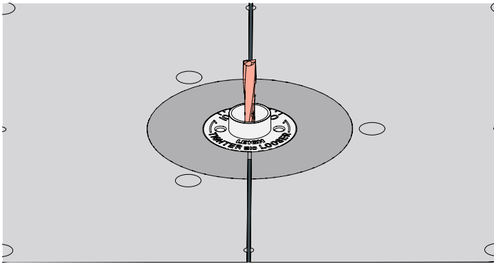
12-8 With the power disconnected from the router, install the optional 3/16" Leigh 166 (HSS) or 166C (solid carbide) bit. Make sure the bit spins freely in the bushing before reconnecting the power. Optional bits available at leighjigs.com
