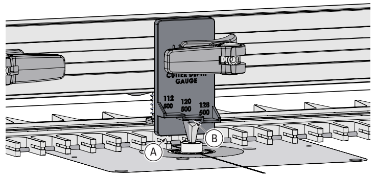
9-13 Bit Height: Clamp the cutter depth gauge as shown, flush on the template (A). Raise the bit until it touches the bottom of the gauge for the selected bit (B). ⚠️ Double check that the bit still rotates freely. Hint: As you raise the bit, slide a piece of paper back and forth until it is trapped and snags on the bit.
