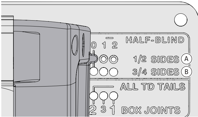
9-10 NOTE: Use the 1/2" SIDES row (A) for tail boards (sides) \frac{3}{8} " [9mm] to \frac{5}{8} " [16mm] thick and the 3/4" SIDES row (B) for tail boards \frac{1}{16} " [17.5mm] to \frac{7}{8} " [22mm] thick.
