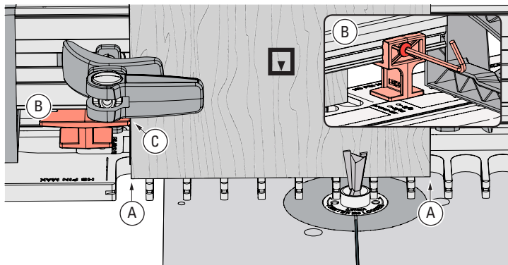
8-10 Center tail board 1 (A) over the template with the marked inside face showing out, bottom end flush on the template, and clamp. From the other side of the frame, slide the side stop (B) to touch the tail board (C) and tighten with the hex driver.
