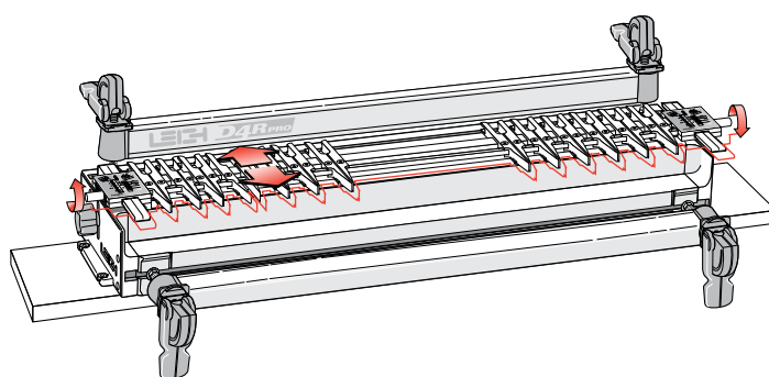
4-2 The guidefinger assembly slides on to the support brackets above the workpiece. The finger assembly is adjusted in or out using calibrated scales on each end to suit different thicknesses of vertical boards.
