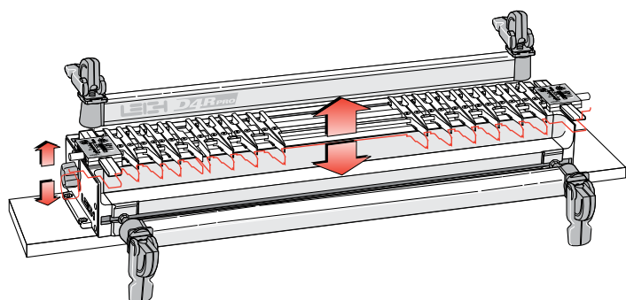
4-3 The finger assembly is raised or lowered using the support brackets to suit different thicknesses of horizontal boards. ■
