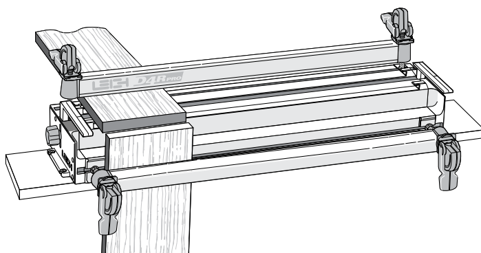
4-1 The two clamp bars hold workpieces horizontally or vertically. The side stops align the boards in the correct position each time.
